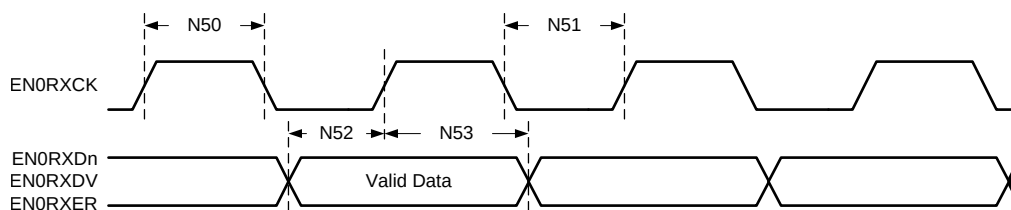
Figure 5-41. 10-Mbps MII Receive Timing
