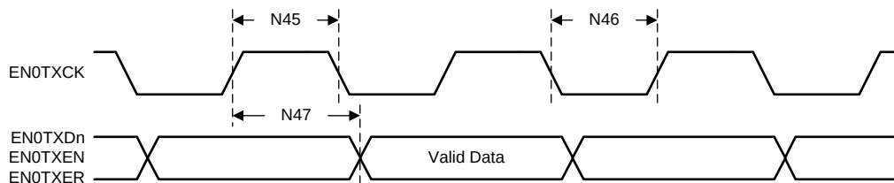
Figure 5-40. 10-Mbps MII Transmit Timing
