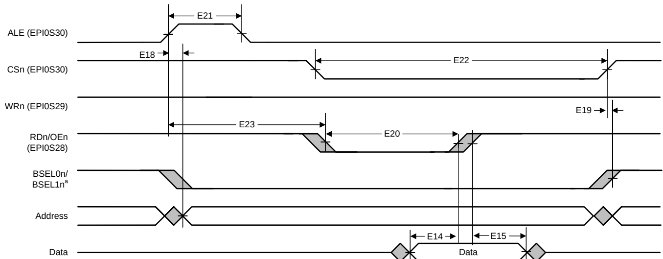
Figure 5-19. Host-Bus 8/16 Asynchronous Mode Read Timing
