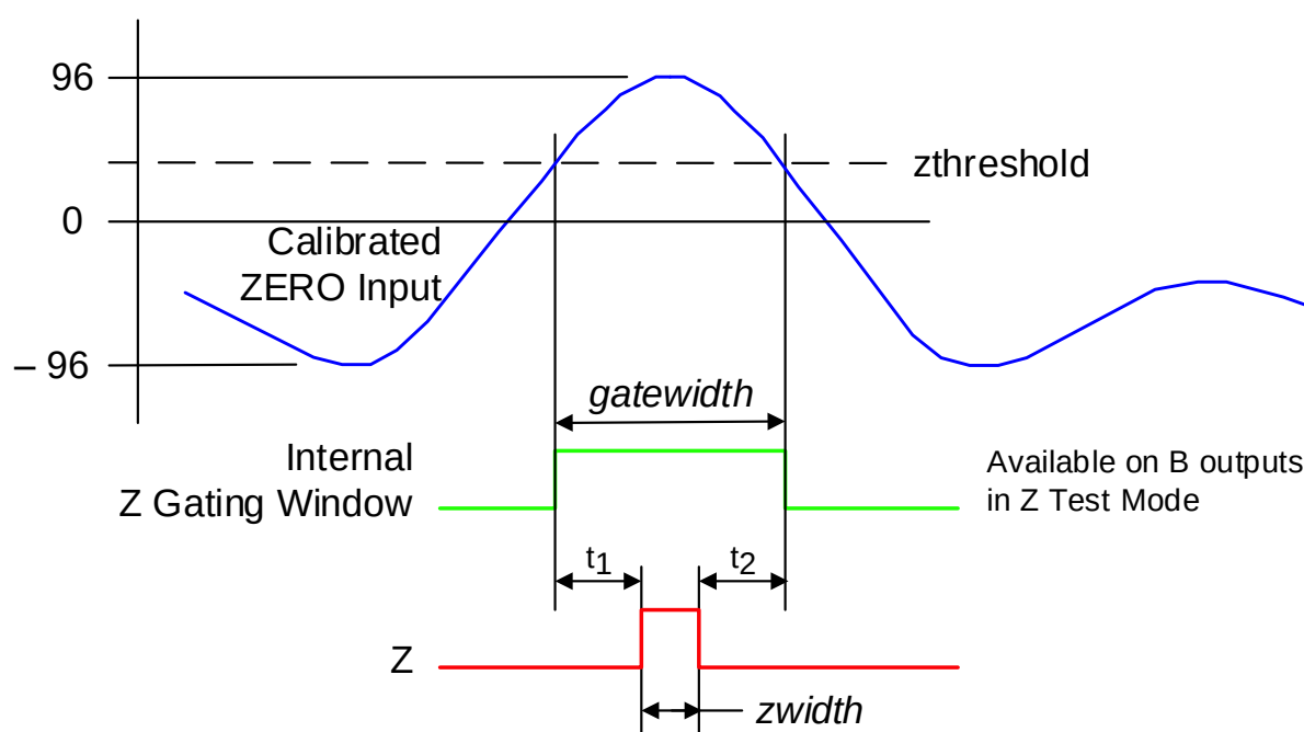
Figure 36: Z Calibration
