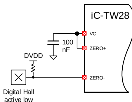
Figure 15: Digital Index Sensor Connection
