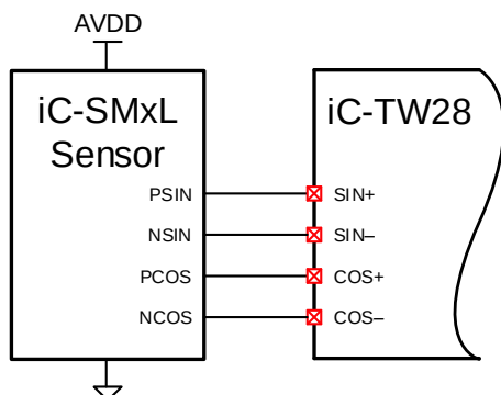
Figure 13: Magnetic Sensor Connection
