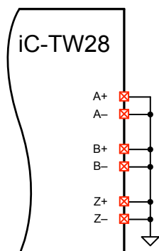
Figure 29: SPI Only Output Connections
