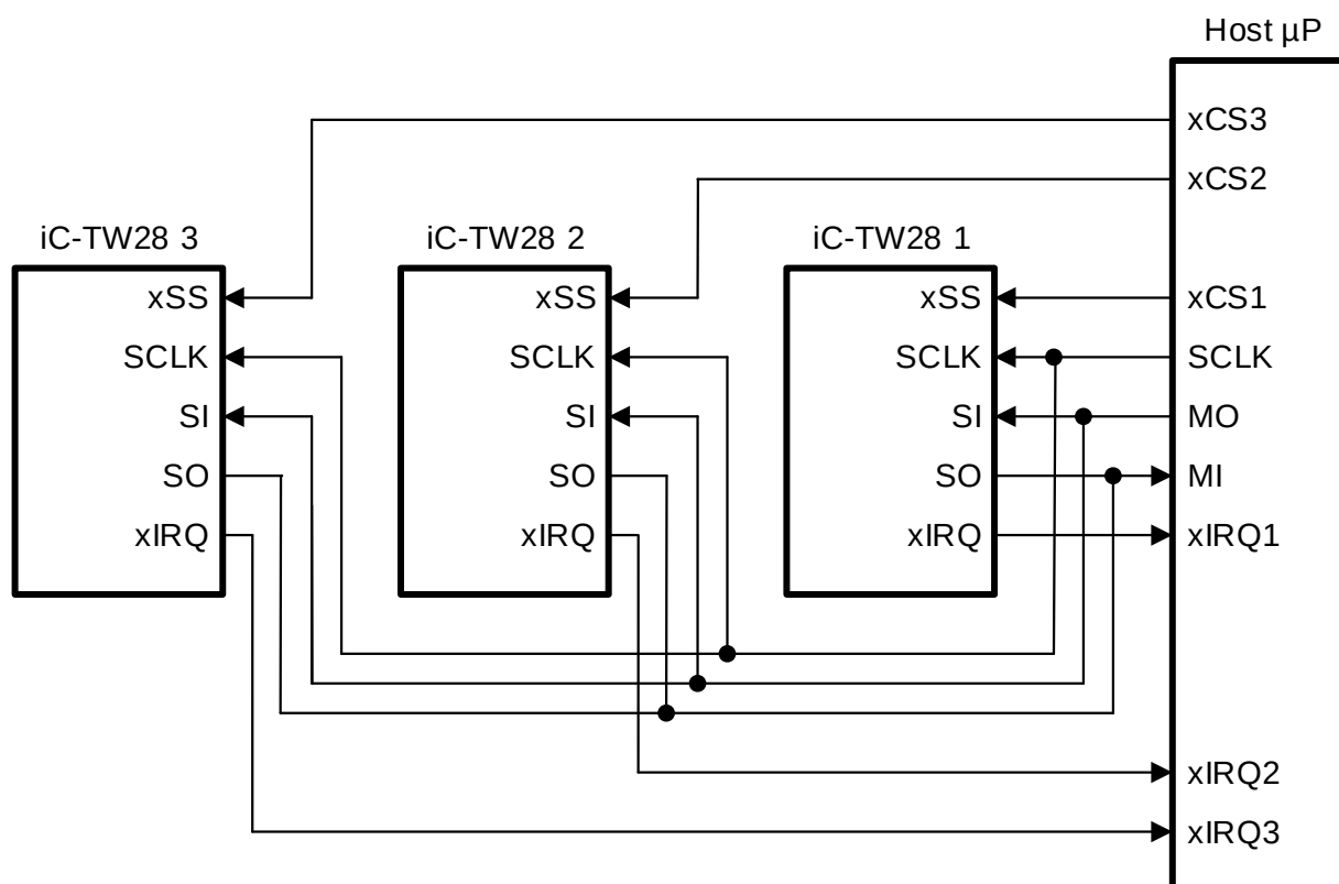
Figure 45: SPI Bus Connection of Multiple iC-TW28s
