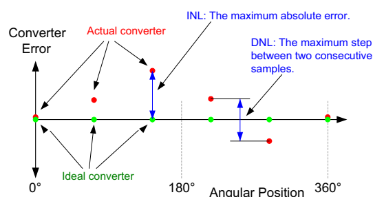
Figure 4: Definition of Integral and Differential Nonlinearity
