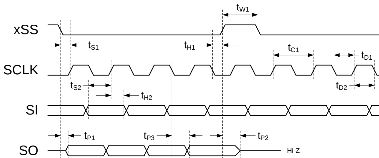
Figure 5: SPI Timing
