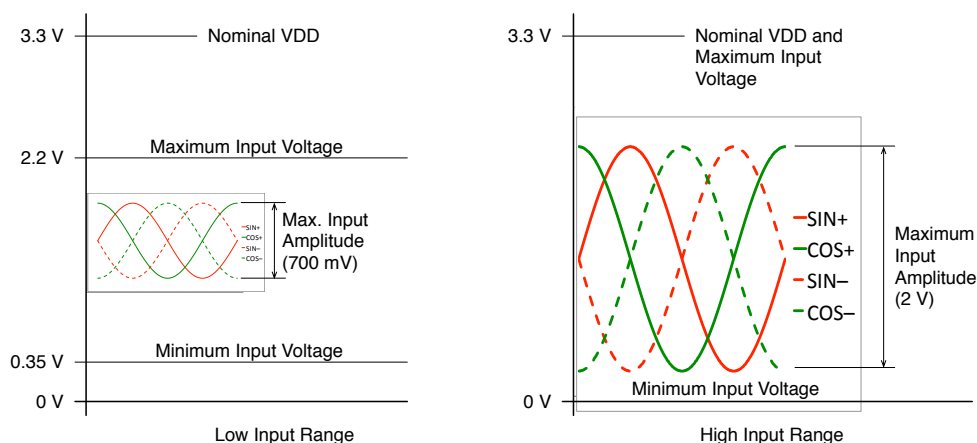
Figure 1: Differential Input Amplitude A_{in}()_{diff} : \text{Max}(\text{SIN}+ - \text{SIN}-) or \text{Max}(\text{COS}+ - \text{COS}-)
