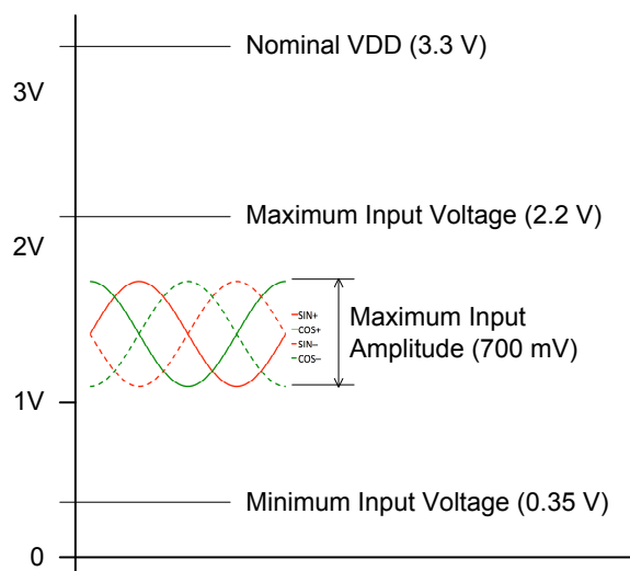
Figure 27: Low Input Range Signals
