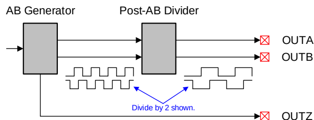
Figure 44: Post-AB Divider
