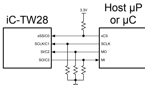
Figure 20: SPI Port Connection
