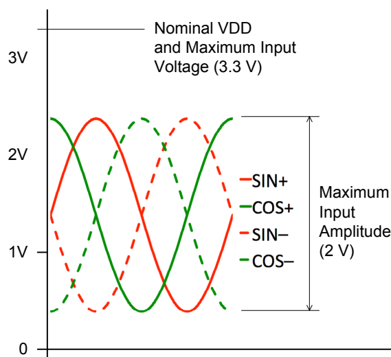
Figure 28: High Input Range Signals
