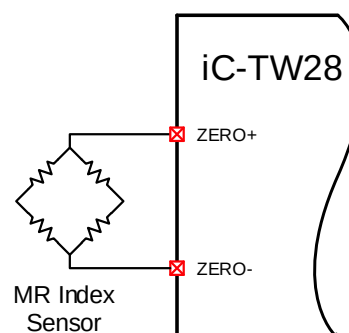
Figure 16: Analog Index Sensor Connection
