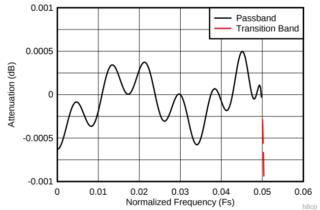
Figure 11. Decimate-by-4 Composite Zoomed Pass-Band Response
